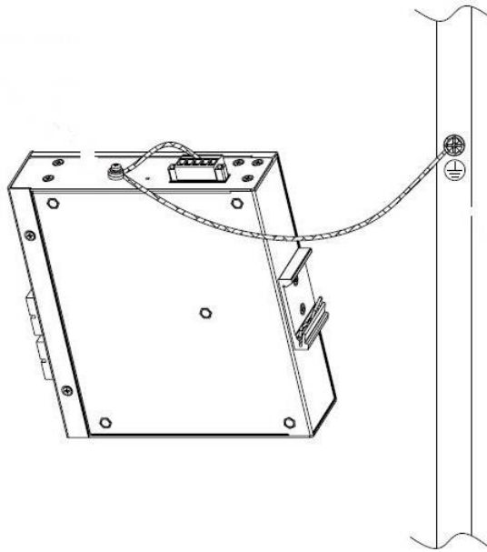
Figure 3-4 track Ground completion schematic
