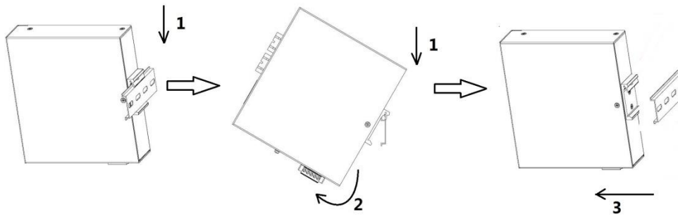
Figure 3-2 track installation diagram
