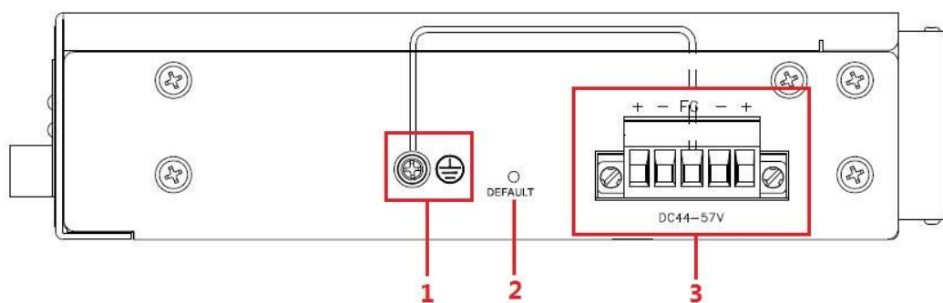
Figure 1-2 Back template of the 8 switch
