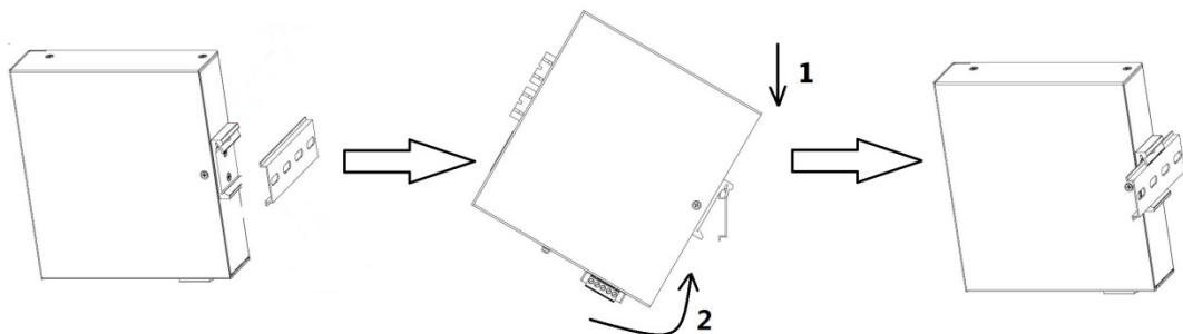
Figure 3-1 track installation diagram
